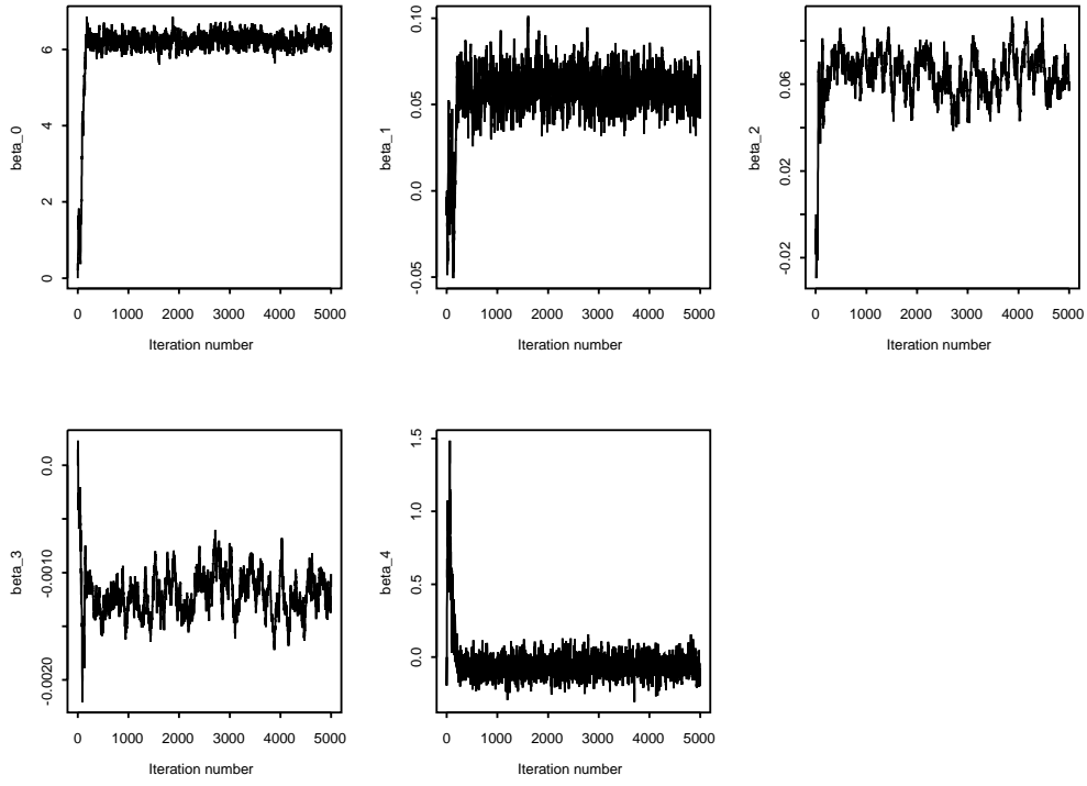
Fig. 1. Time series plot of five model parameters based on 5000 iterations from Metropolis algorithm.
